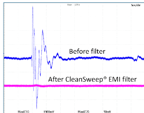
Typical Performance with Differential Mode Noise
